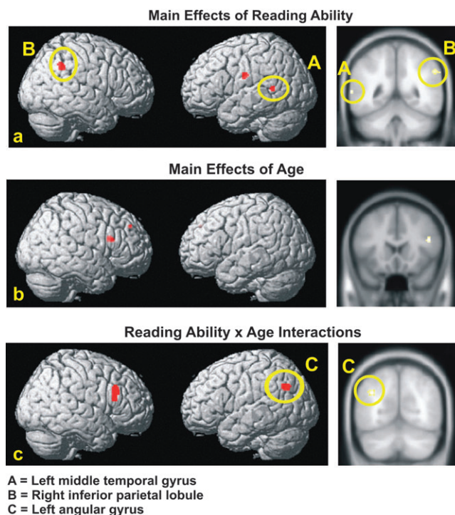
Figure 2. Multiple regression analyses: Main effects of reading ability, age, and age × reading ability interaction. Top row (panel a) presents surface rendering and canonical view of regions correlated with reading ability. Middle row (panel b) presents surface rendering and canonical view of regions correlated with age. Bottom row (panel c) shows surface rendering of regions and canonical view showing age × reading ability interaction. Yellow ovals encircle parietotemporal activation.
